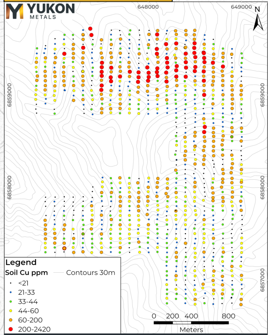
COPPER-IN-SOILS AT BIRCH 50M X 100M GRID.
